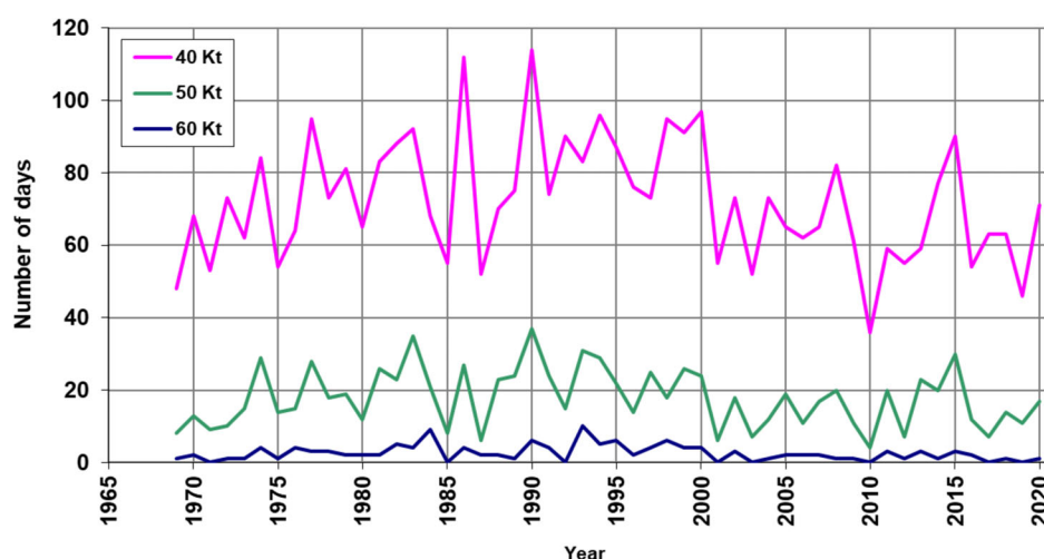
FIGURE 40 Count of the number of individual days each year during which a max gust speed \geq 40 , 50 and 60 Kt (46, 58, 69 mph; 74, 93, 111 kph) has been recorded by at least 20 or more UK stations, from 1969 to 2020. Stations above 500 m above sea level are excluded
