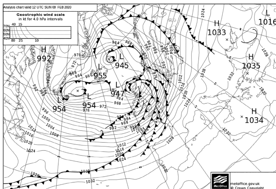
FIGURE 43 Analysis chart at 1200 UTC 9 February 2020
