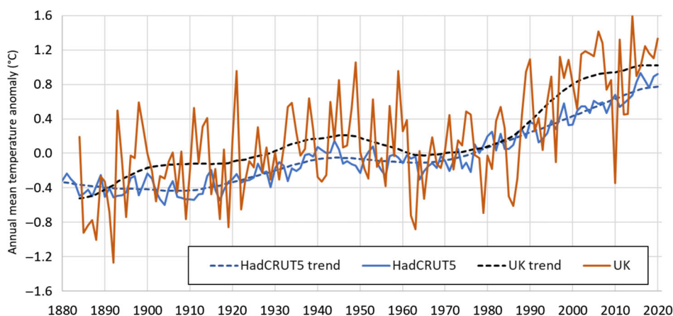
FIGURE 12 Annual T_{\text{mean}} ( ^{\circ}\text{C} ) for the UK, 1884–2020, plotted alongside global annual T_{\text{mean}} ( ^{\circ}\text{C} ) based on HadCRUT5 dataset. Both series are expressed as anomalies relative to the 1961–1990 average
