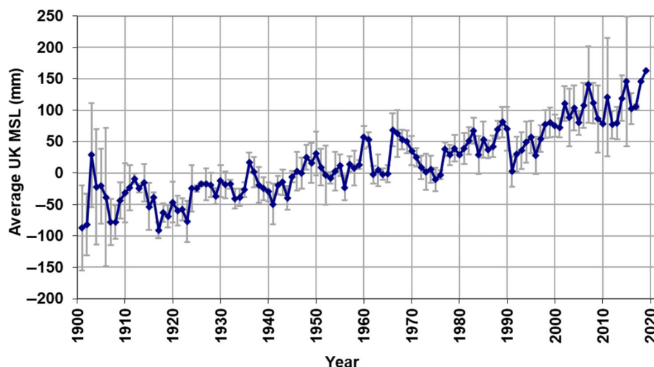
FIGURE 41 UK sea level index for the period since 1901 computed from sea level data from five stations (Aberdeen, North Shields, Sheerness, Newlyn and Liverpool) from Woodworth et al. (2009). Error bars shown in the UK index indicate uncertainty (one standard deviation) in values for individual years
