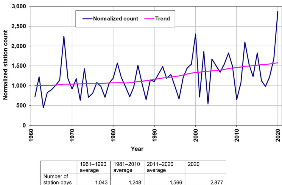
FIGURE 33 Annual count of the number of UK station-days which have recorded daily rainfall totals greater than or equal to 50 mm from 1961 to 2020, adjusted for station network size and excluding stations above 500 m above sea level. The table provides average annual values (station-days). Note that the number of station-days for the 1961–1990 and 1981–2010 averages has changed slightly from last year’s report (1,050, 1,256). This is because the adjustment for station network size has altered as a result of inclusion of year 2020. However, historical observations held within the climatological database also change over time as more digitized data are added or as a result of quality control; data for the full series have been re-extracted from this live database
