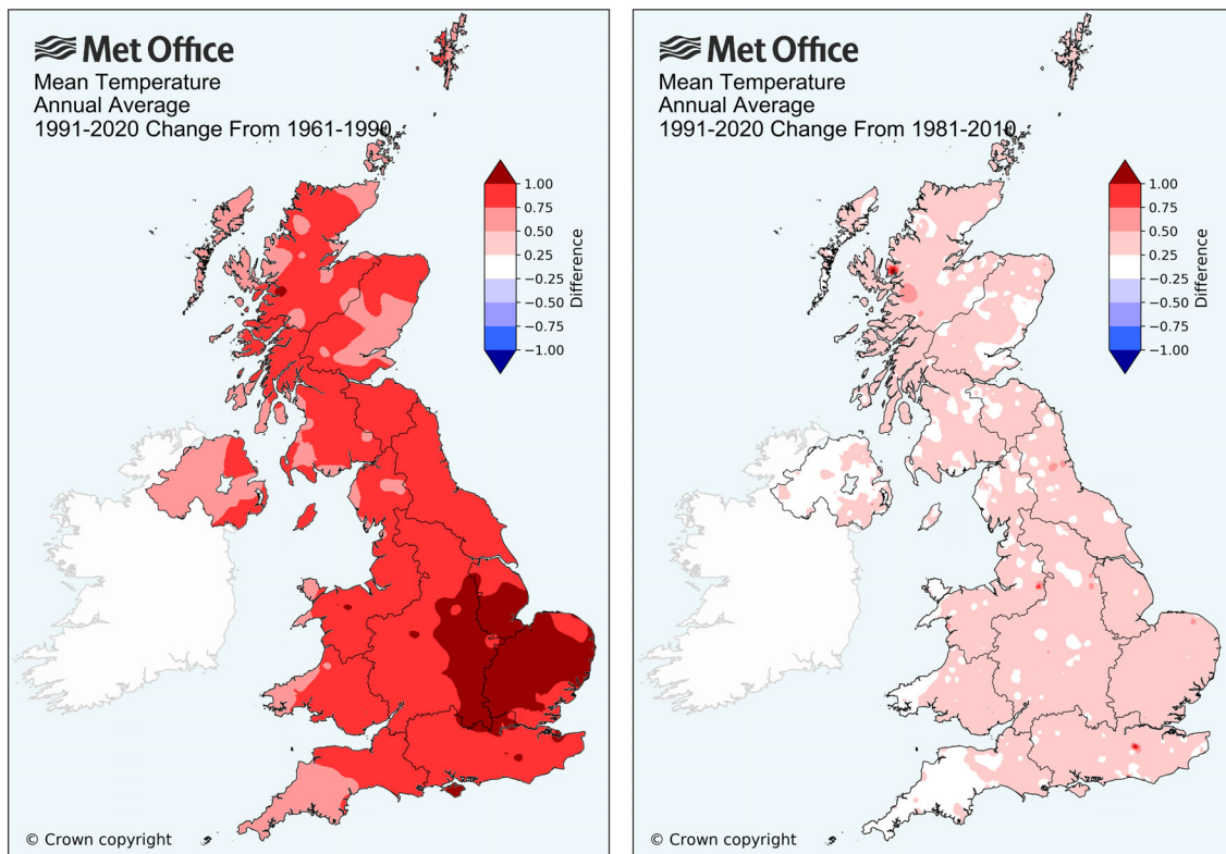
FIGURE 70 Difference ( ^{\circ}\text{C} ) between preliminary 1991–2020 annual average T_{\text{mean}} and earlier periods 1961–1990 and 1981–2010
