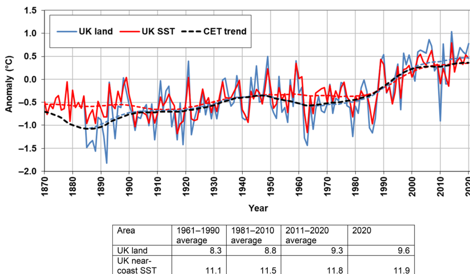
FIGURE 21 UK annual mean temperature over land 1884–2020, Central England temperature trend and UK annual mean sea surface temperature across near-coastal waters around the UK 1870–2020 (°C), expressed as anomalies relative to the 1981–2010 long-term average. Hatched blue and red lines are the UK land and SST trends. The table provides average annual values (°C)
