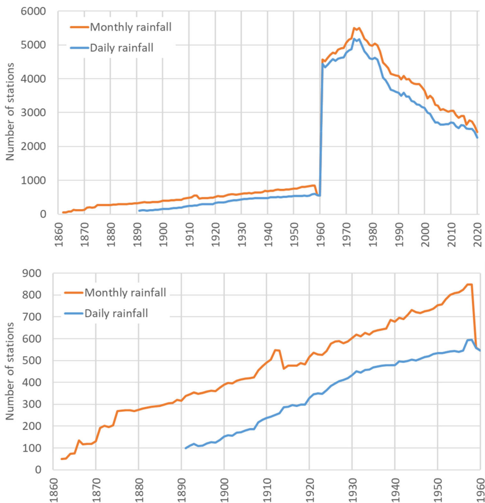
FIGURE A1.2 Number of stations used for monthly/daily rainfall (a) 1862/1891–2020 and (b) 1862/1891–1960, with the step change from <1,000 stations to >4,000 stations occurring in 1961
