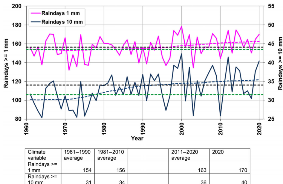
FIGURE 30 Annual average number of days of rain \geq 1 and 10 mm for the UK, 1961–2020. The hatched black line is the 1981–2010 long-term average. The hatched green line is the 1961–1990 long-term average. The table provides average annual values (days)
