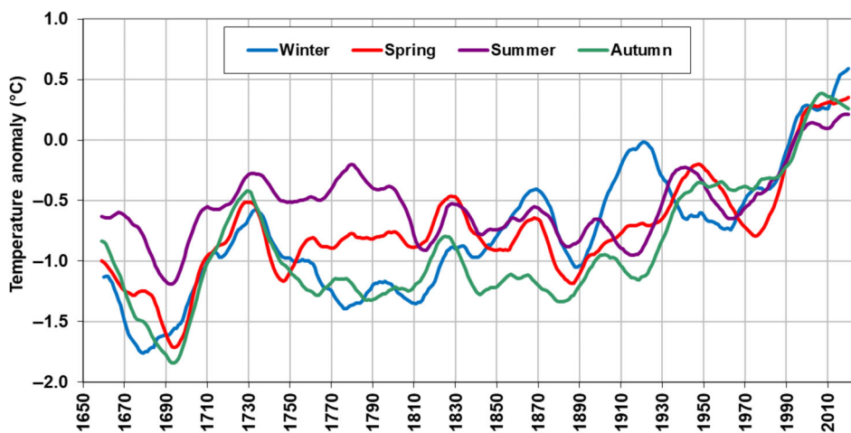
FIGURE 11 Seasonal CET series ( ^{\circ}\text{C} ), 1659–2020, expressed as anomalies relative to 1981–2010 average. The figure shows a smoothed trend for each series using a weighted kernel filter described in Annex 2
