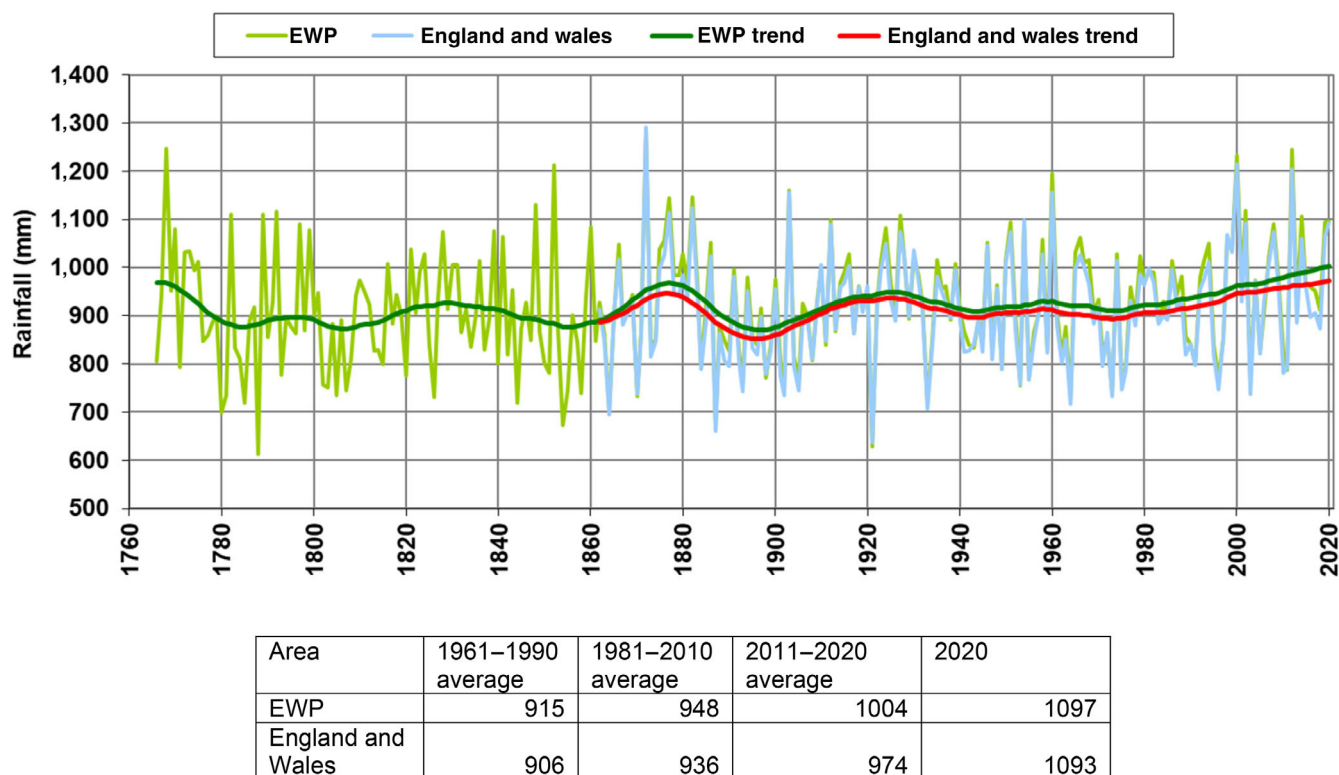
FIGURE 27 Annual rainfall for EWP series, 1766–2020, and England and Wales areal series, 1862–2020 (mm). The table provides average annual rainfall values (mm)
