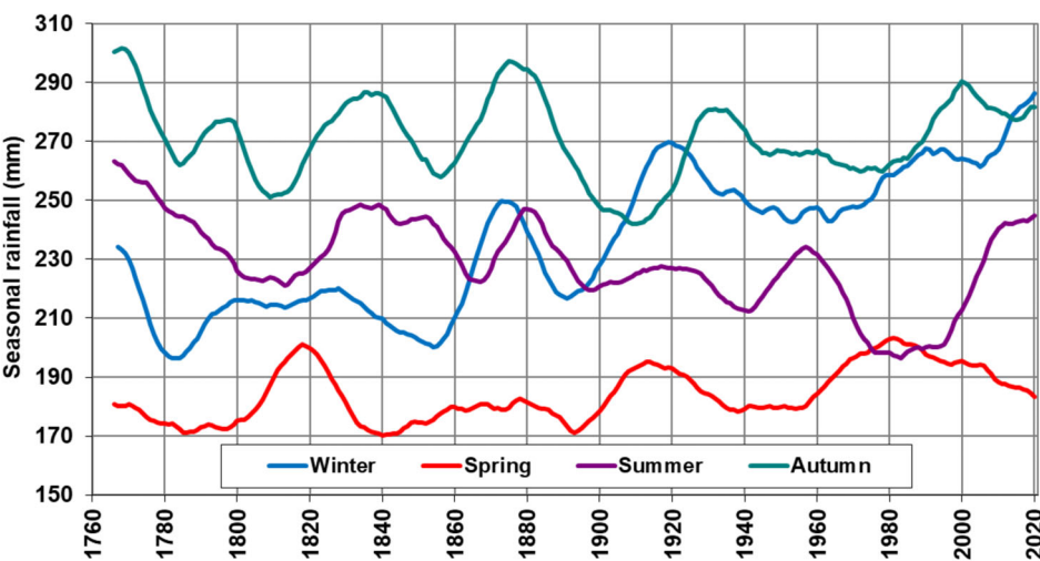
FIGURE 28 Seasonal rainfall trends for EWP series in mm, 1766–2020 (note winter from 1767). The figure shows a smoothing trend for each series using a weighted filter (see Annex 2)
