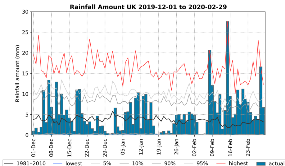
FIGURE 49 UK daily area-average rainfall totals for winter 2020 (December 2019–February 2020)
