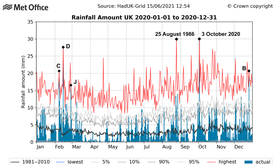
FIGURE 69 UK area-average daily rainfall during 2020. The wettest days are labelled: C—storm Ciara, D—storm Dennis, J—storm Jorge, B—storm Bella, and 3 October 2020. For reference 25 August 1986 is also shown
