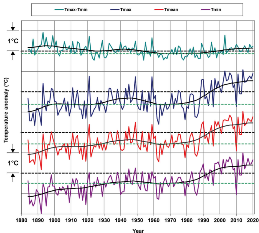
FIGURE 9 Annual T_{\max} , T_{\text{mean}} and T_{\min} ( ^{\circ}\text{C} ) for the UK, and T_{\max} minus T_{\min} , 1884–2020, expressed as anomalies relative to the 1981–2010 average. The hatched black line is the 1981–2010 long-term average. The lower hatched green line is the 1961–1990 long-term average. Light grey grid-lines represent anomalies of \pm 1^{\circ}\text{C} . The table provides average absolute values ( ^{\circ}\text{C} )
