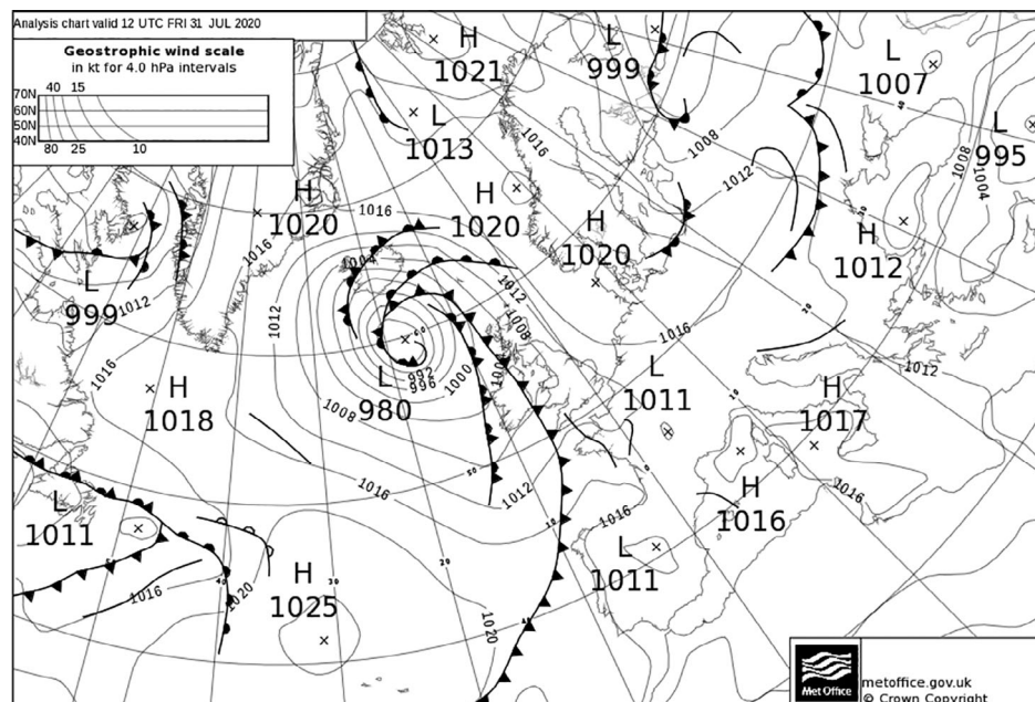
FIGURE 55 Analysis chart at 1200 UTC 31 July 2020
