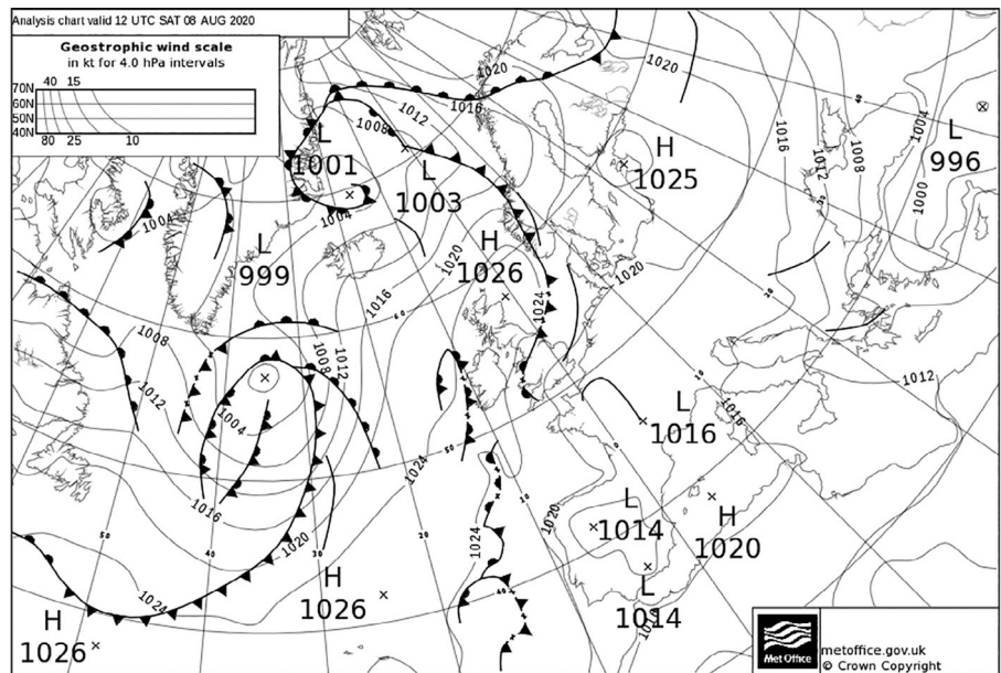
FIGURE 58 Analysis chart at 1200 UTC 8 August 2020
