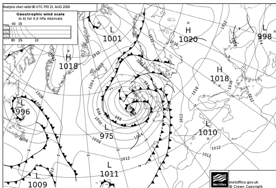
FIGURE 64 Analysis chart at 0600 UTC 21 August 2020
