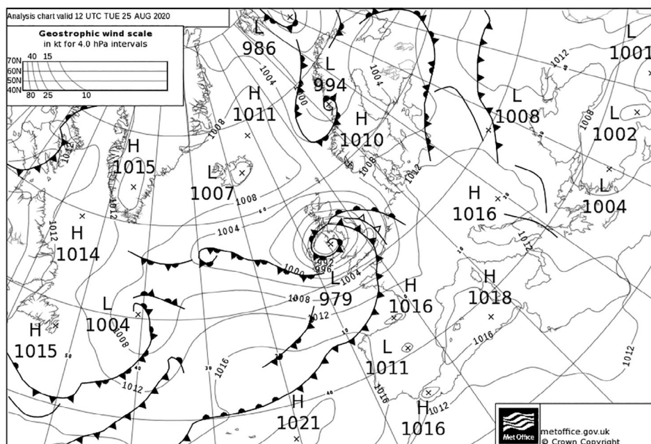
FIGURE 65 Analysis chart at 1200 UTC 25 August 2020
